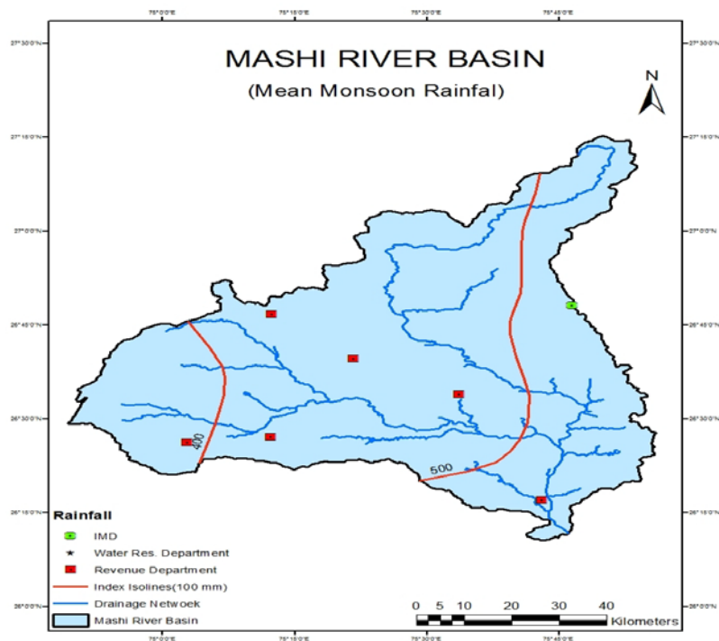
Figure 10: Mean Monsoon Rainfall in Mashi River Basin
