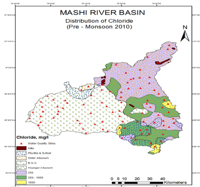
Figure 16: Location of Chloride in groundwater in Mashi Sub Basin
