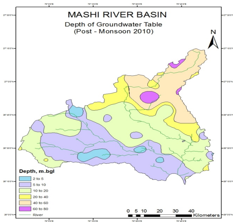
Figure 12: Depth of groundwater table- Post Monsoon
