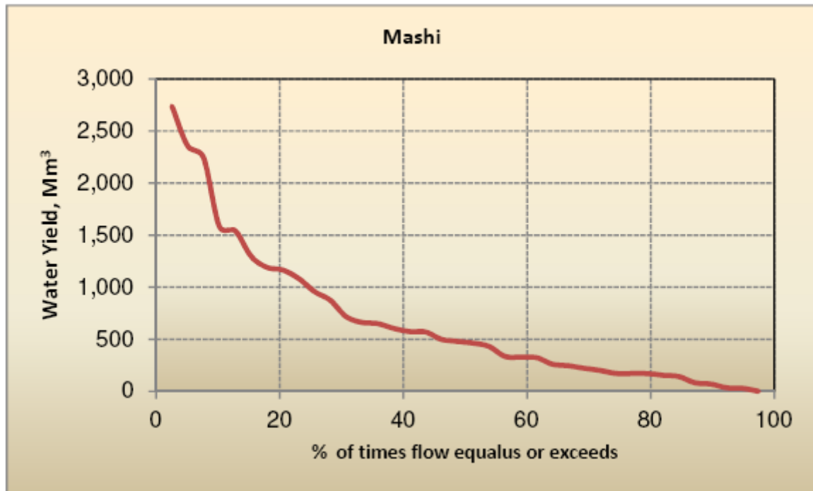
Figure 8: Simulated Flow Duration Curves for Mashi Sub-basin of Banas River Basin
