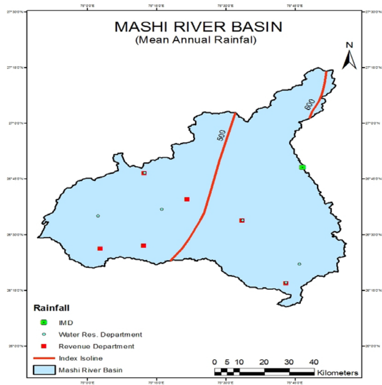
Figure 9: Mean Annual rainfall in Mashi River Basin
