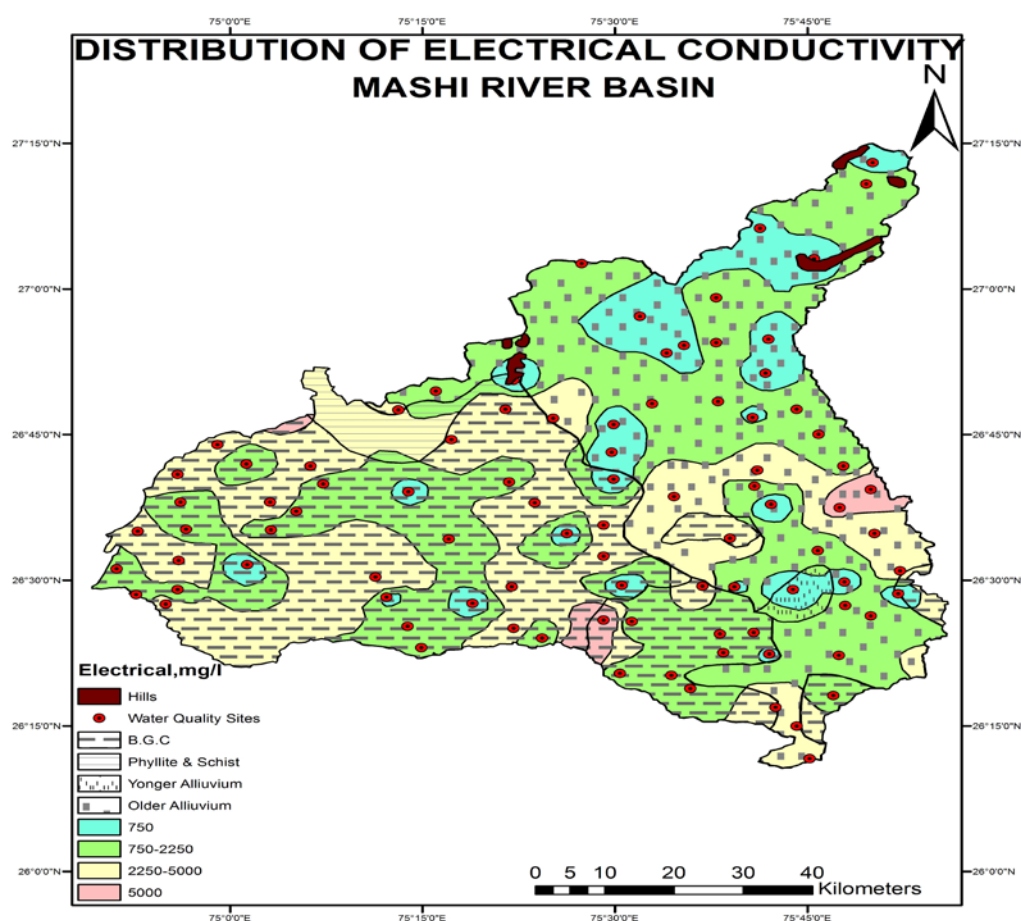
Figure 19: Distribution of EC of Groundwater in Mashi Sub Basin.
