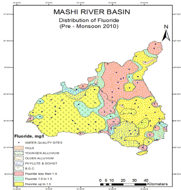
Figure 17: Location of Fluoride in groundwater in Mashi Sub Basin
