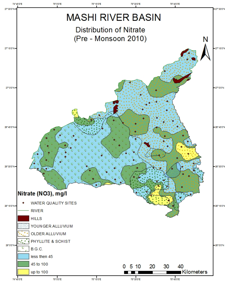
Figure 18: Location of Nitrate in groundwater in Mashi Sub Basin
